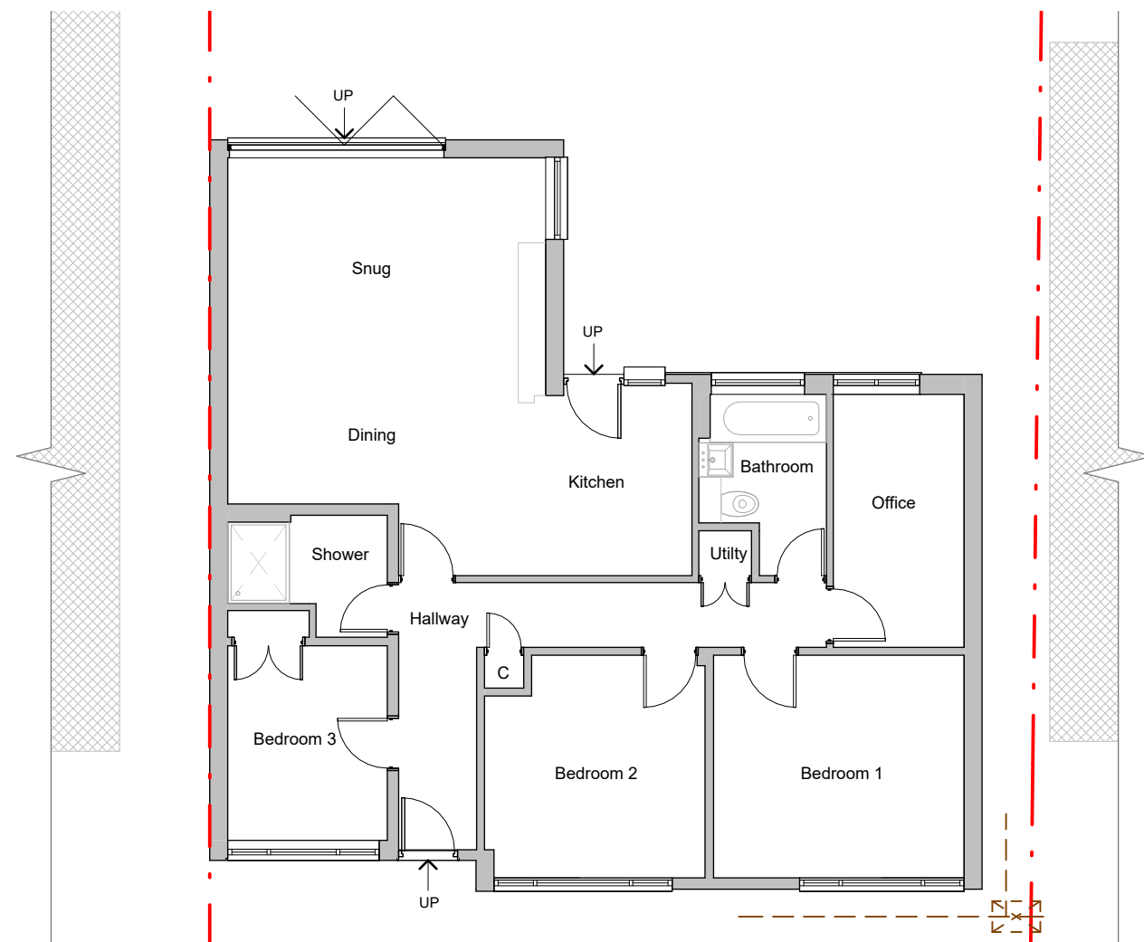
Ground Floor
