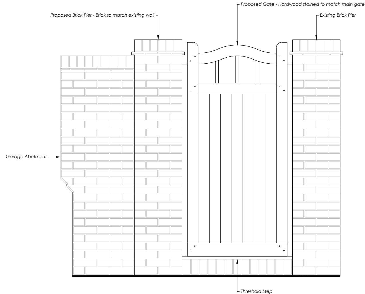
Proposed Gate - Detail B
