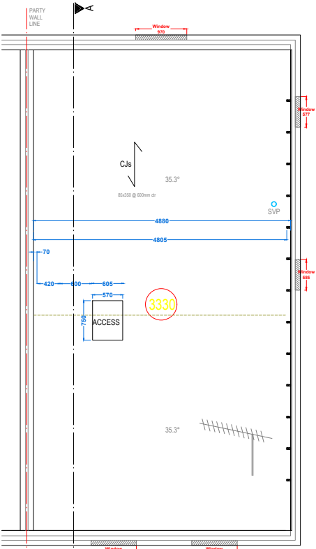
EXISTING LOFT FLOOR PLAN
