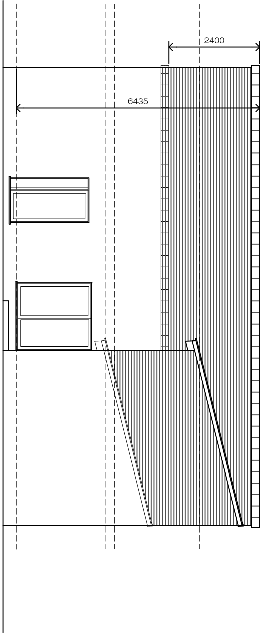
Elevation facing No 3 (side)
