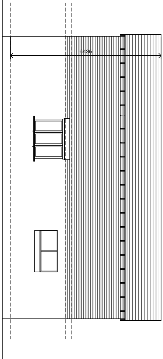
Elevation to Sellafeld Way (side)
