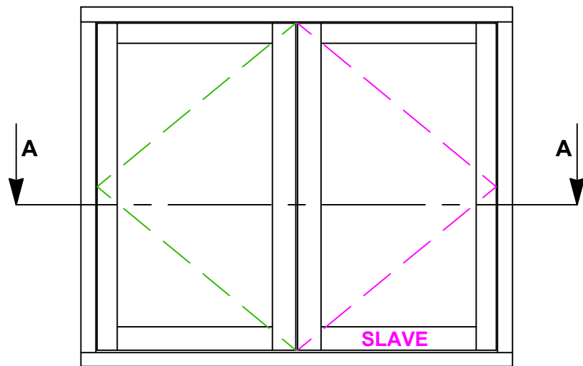
TYPICAL CASEMENT LAYOUT
