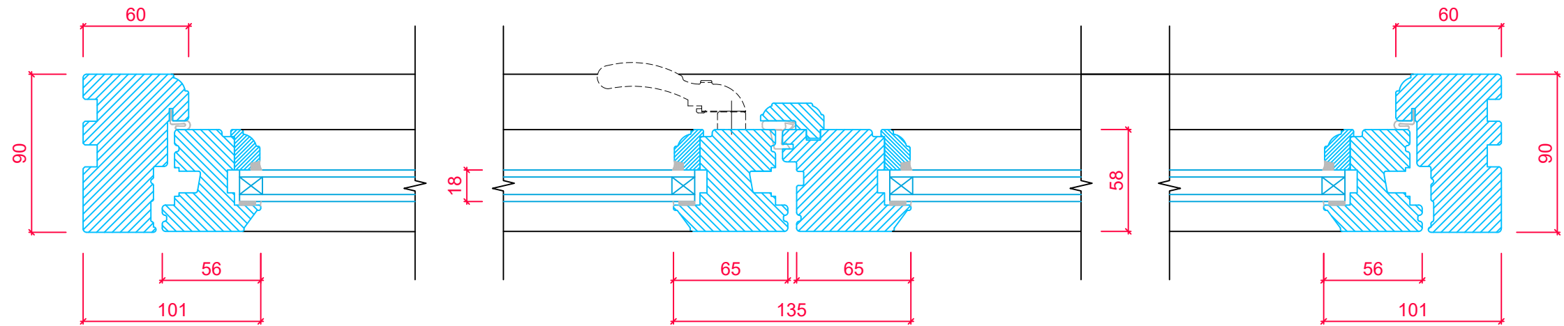
CASEMENT CROSS SECTION 'A-A'
