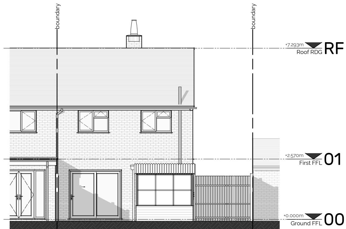
NE | EXISTING NORTH-EAST ELEVATION Scale 1 : 100
