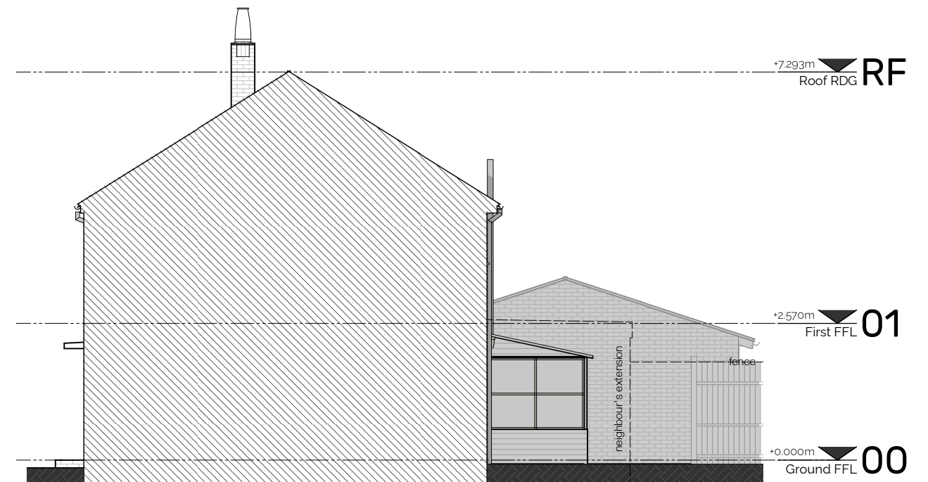
SE | EXISTING SOUTH-EAST ELEVATION Scale 1 : 100
