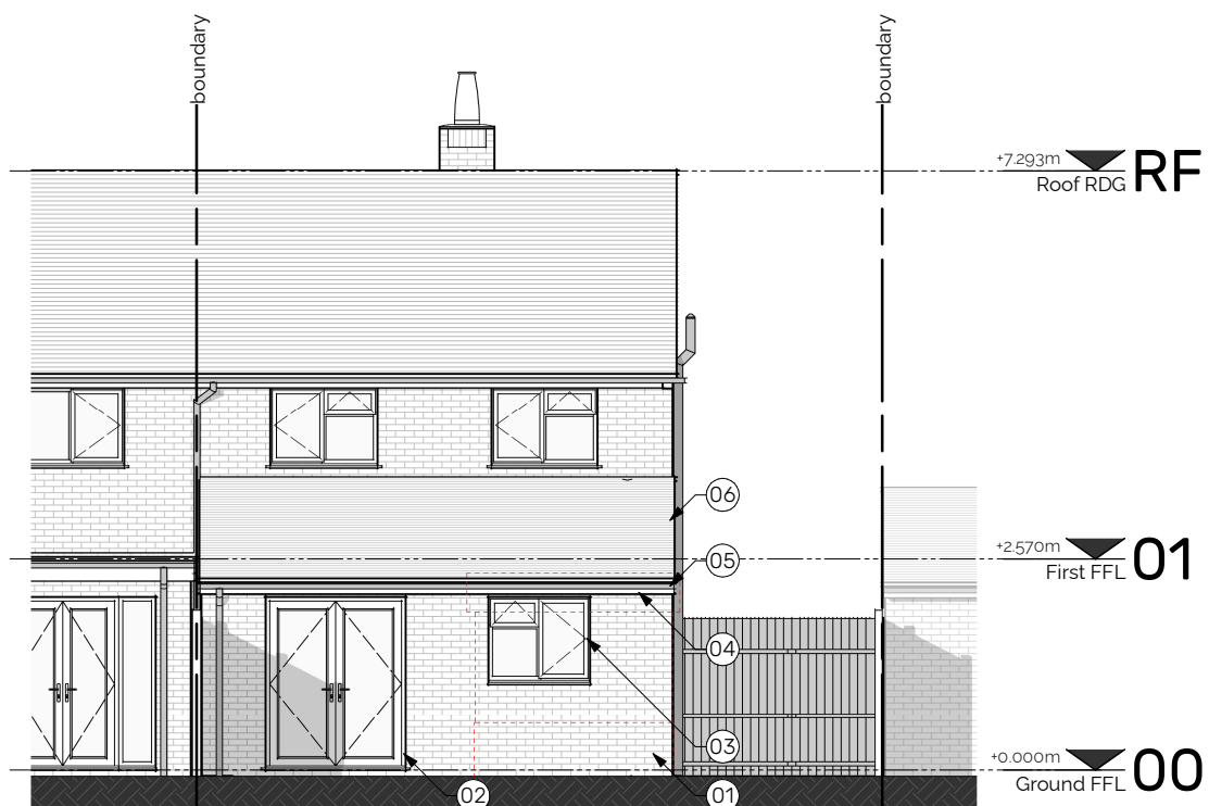
NE | PROPOSED NORTH-EAST ELEVATION Scale 1 : 100
