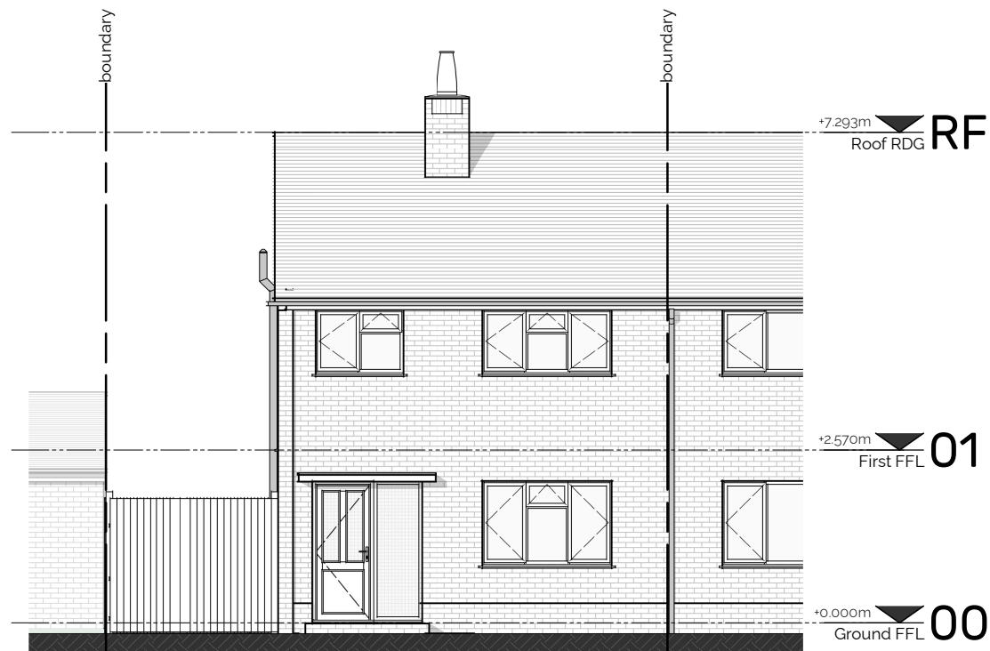
SW | PROPOSED SOUTH-WEST ELEVATION Scale 1 : 100
