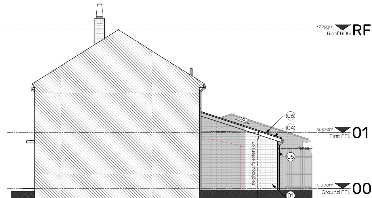
SE | PROPOSED SOUTH-EAST ELEVATION Scale 1 : 100
