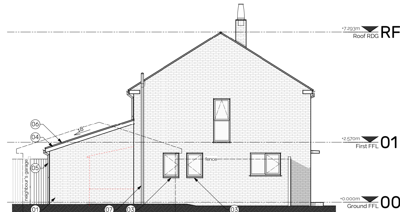
NW | PROPOSED NORTH-WEST ELEVATION Scale 1 : 100
