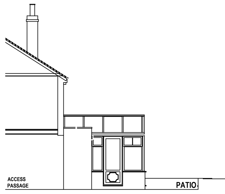
EXISTING WEST ELEVATION
