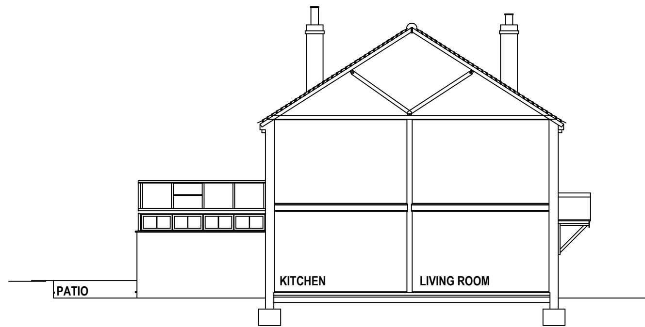
EXISTING EAST ELEVATION - SECTION BB
