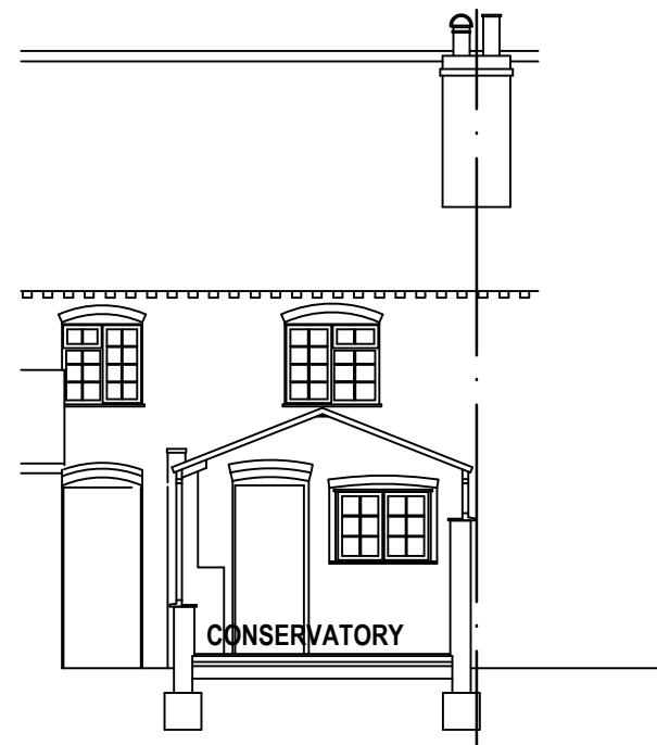
EXISTING SECTION AA
