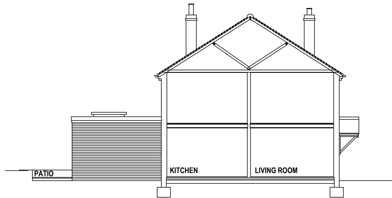
PROPOSED EAST ELEVATION - SECTION BB
