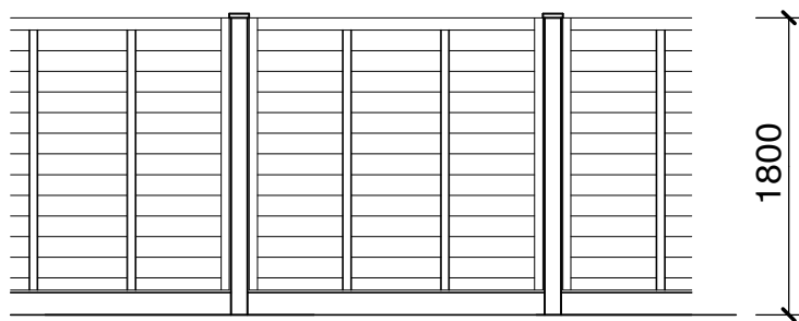
Proposed fence panel 1:50
