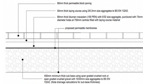
Typical Permeable Paving Construction Detail
