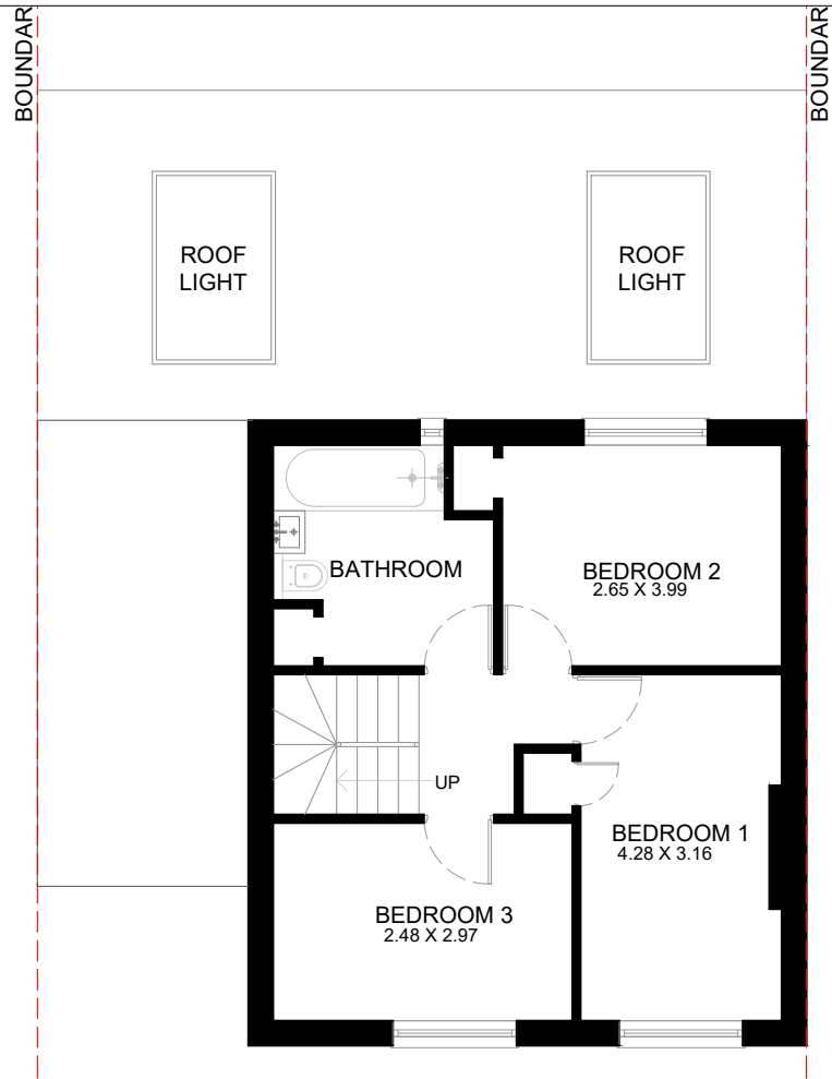
PROPOSED FIRST FLOOR PLAN (1:100 @ A3)
