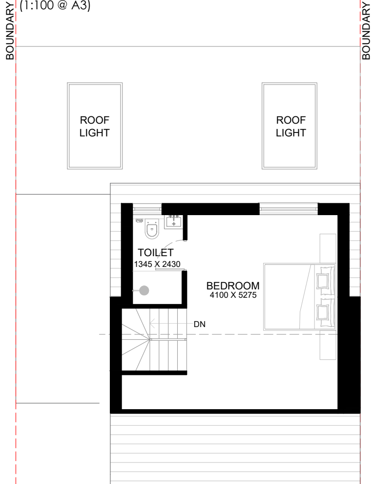
PROPOSED LOFT FLOOR PLAN (1:100 @ A3)
