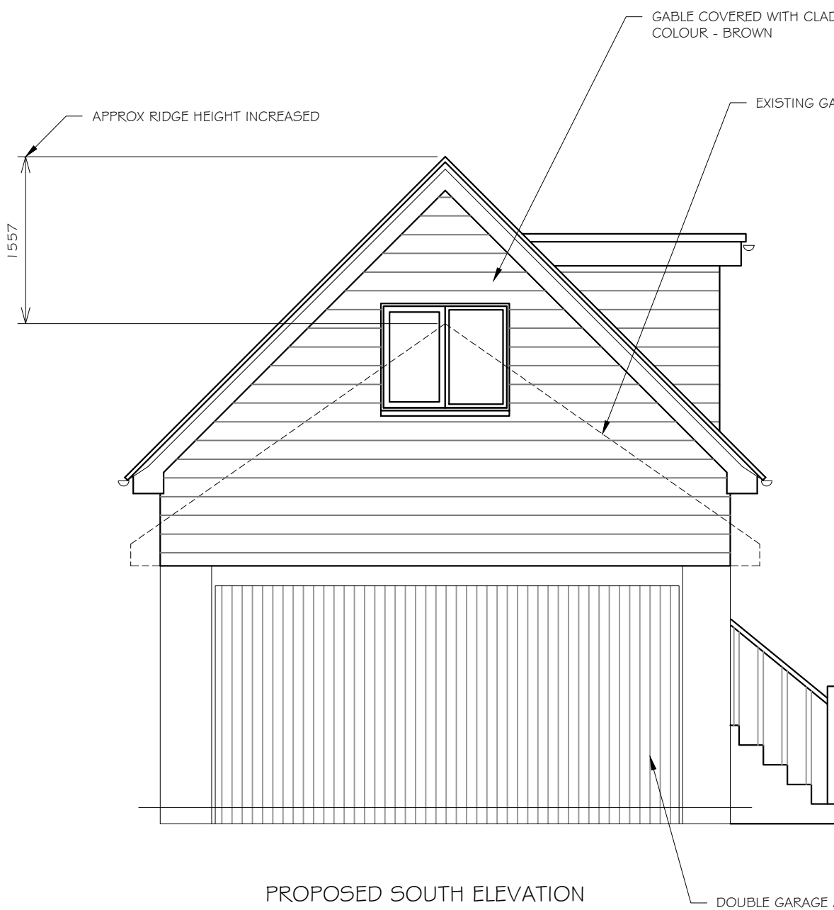
PROPOSED SOUTH ELEVATION
