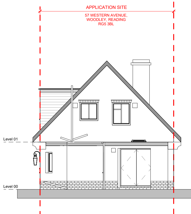
3 EXISTING REAR ELEVATION 1:100
