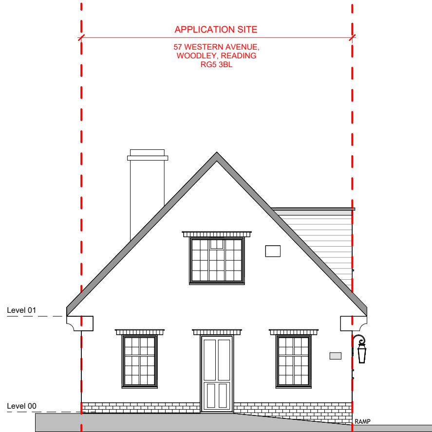
1 EXISTING FRONT ELEVATION (Not intervention) 1:100
