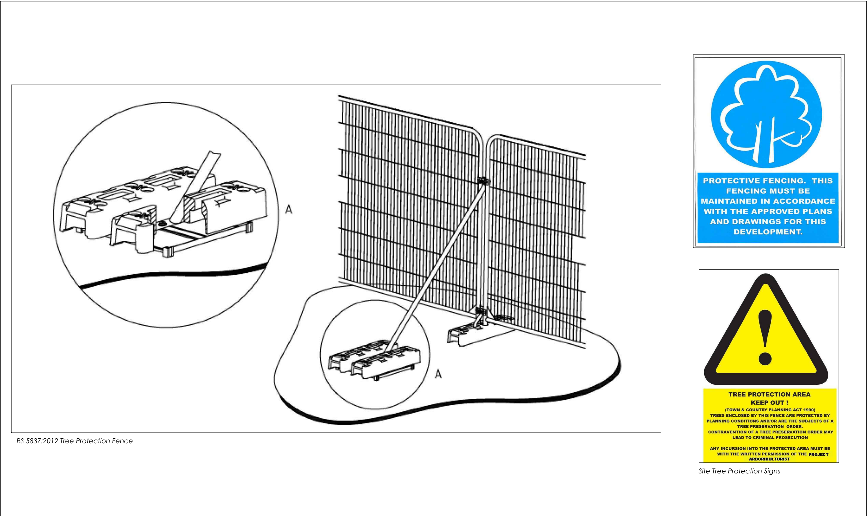
Tree Protection Details - Not to Scale
