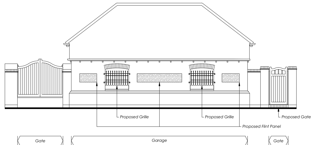
Proposed Street Elevation - Pearson Road
