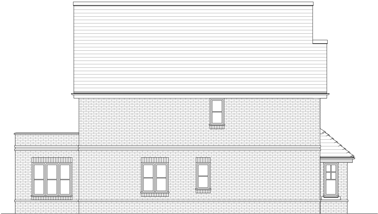
SIDE ELEVATION
