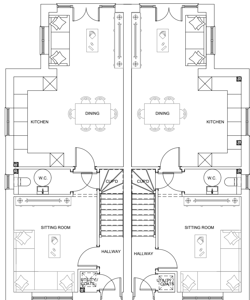
GROUND FLOOR PLAN 1063 SQFT
