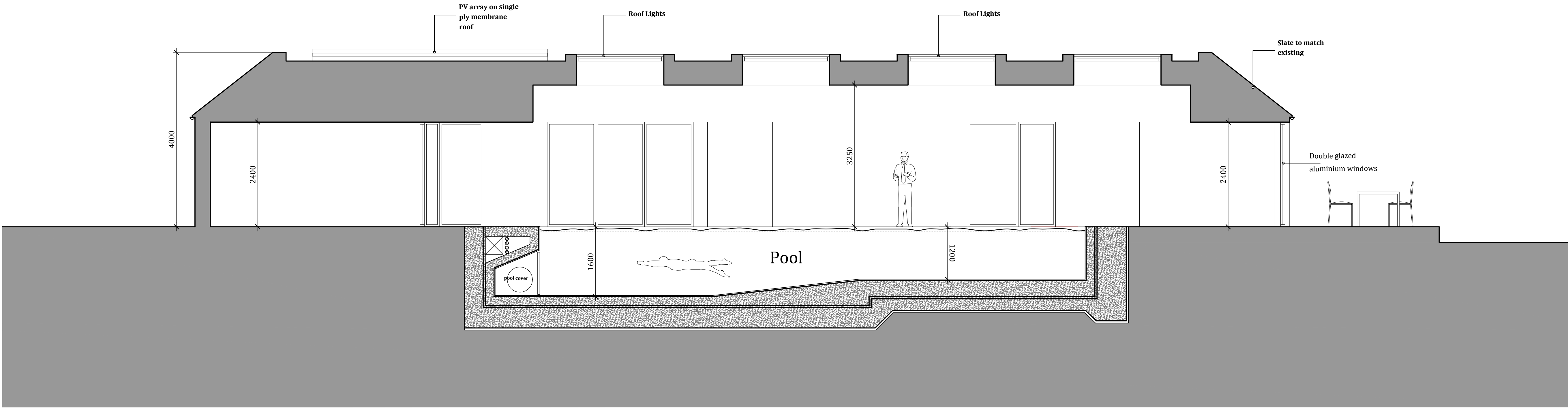
SECTION B-B
