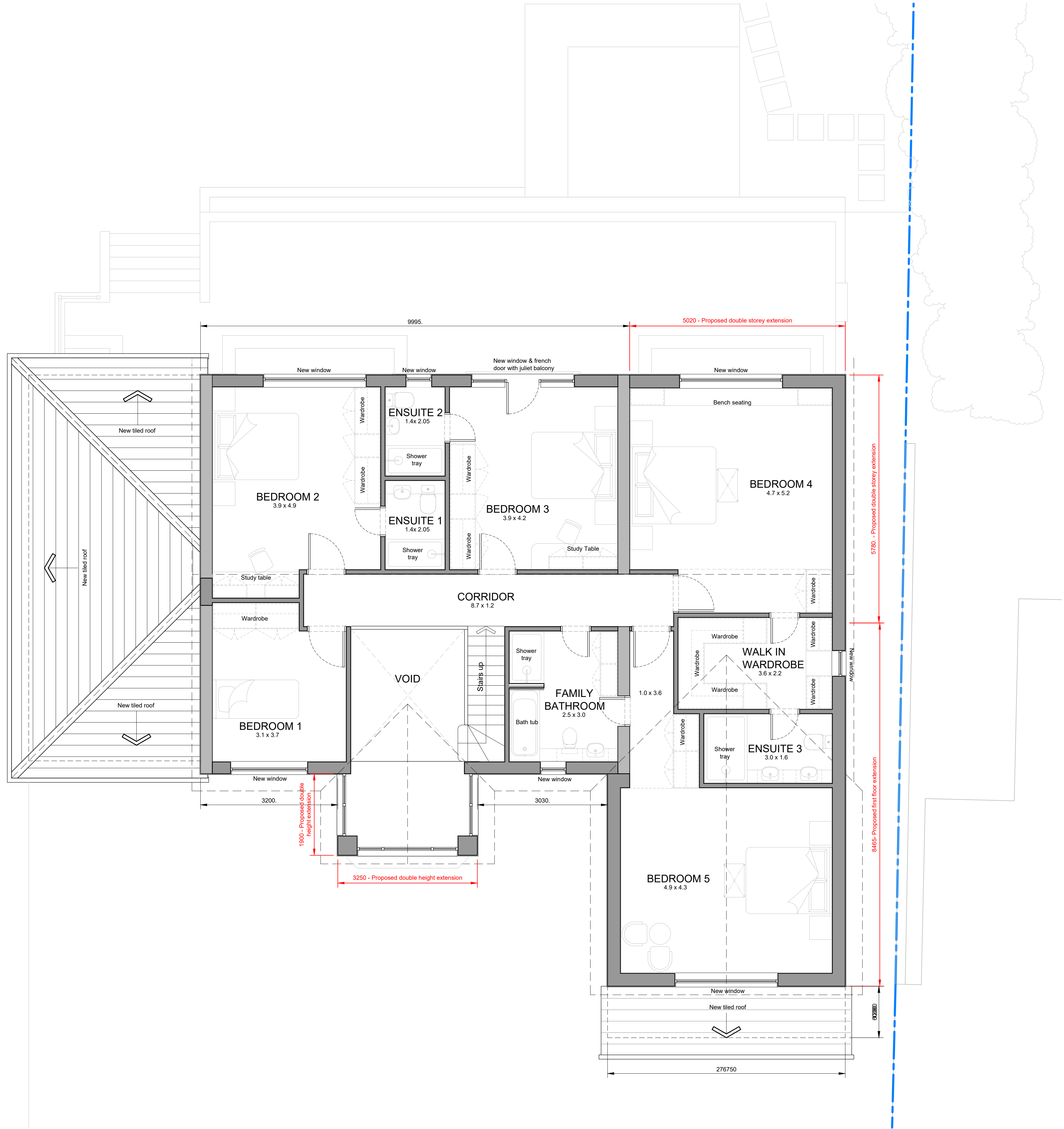
PROPOSED FIRST FLOOR PLAN
