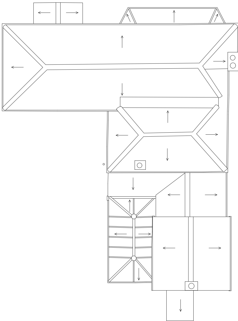
ROOF PLAN
