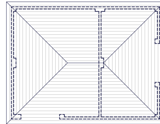
ROOF PLAN
