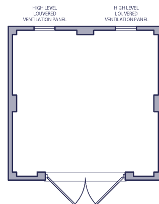
FLOOR PLAN
