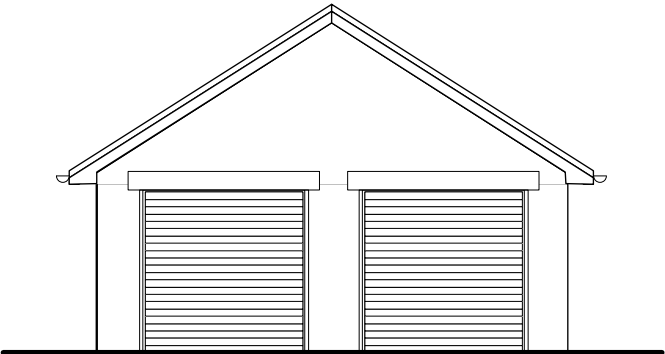
FRONT/NORTH ELEVATION
