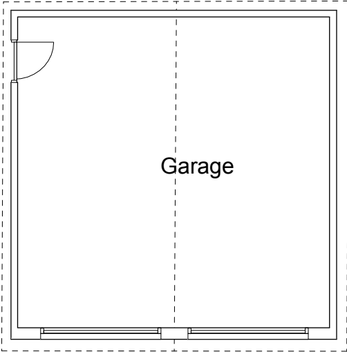
PLAN GEA 39.2m2
