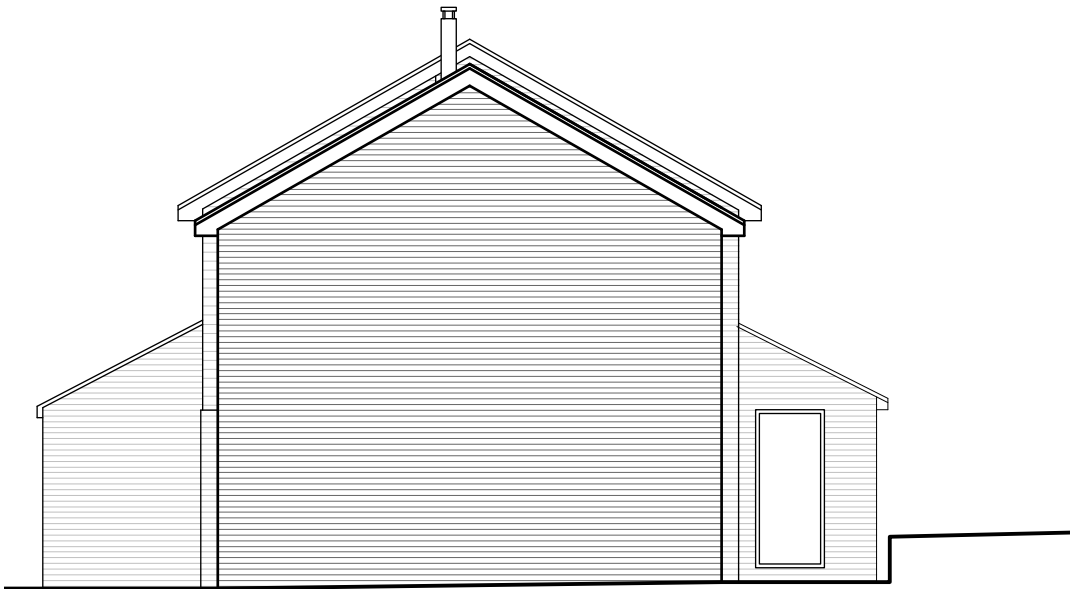
Proposed Side 2 (South) Elevation
