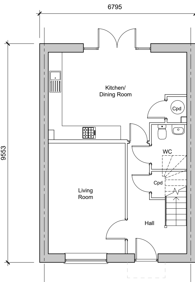
Ground Floor Plan 4-Bedroom House 106.27sqm / 1143.92sqft GIA (to include) Plots - 7 Handed - 8
