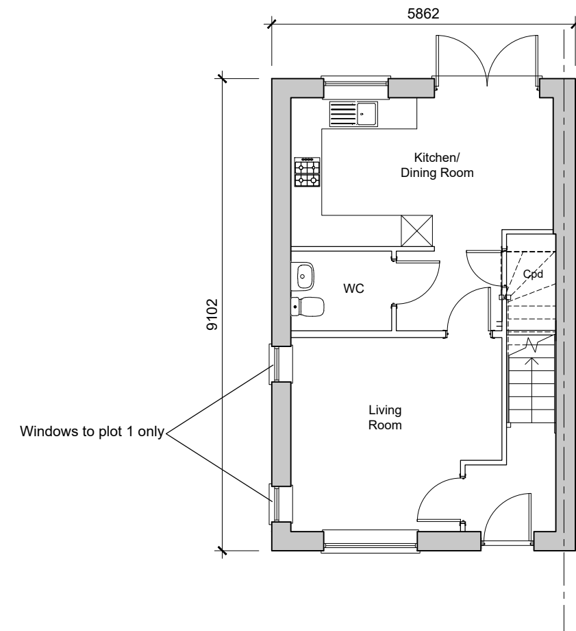
Ground Floor Plan 4-Bedroom House 111.32sqm / 1198.25sqft GIA (approximate) Plots - 1, 3 Handed - 2, 4
