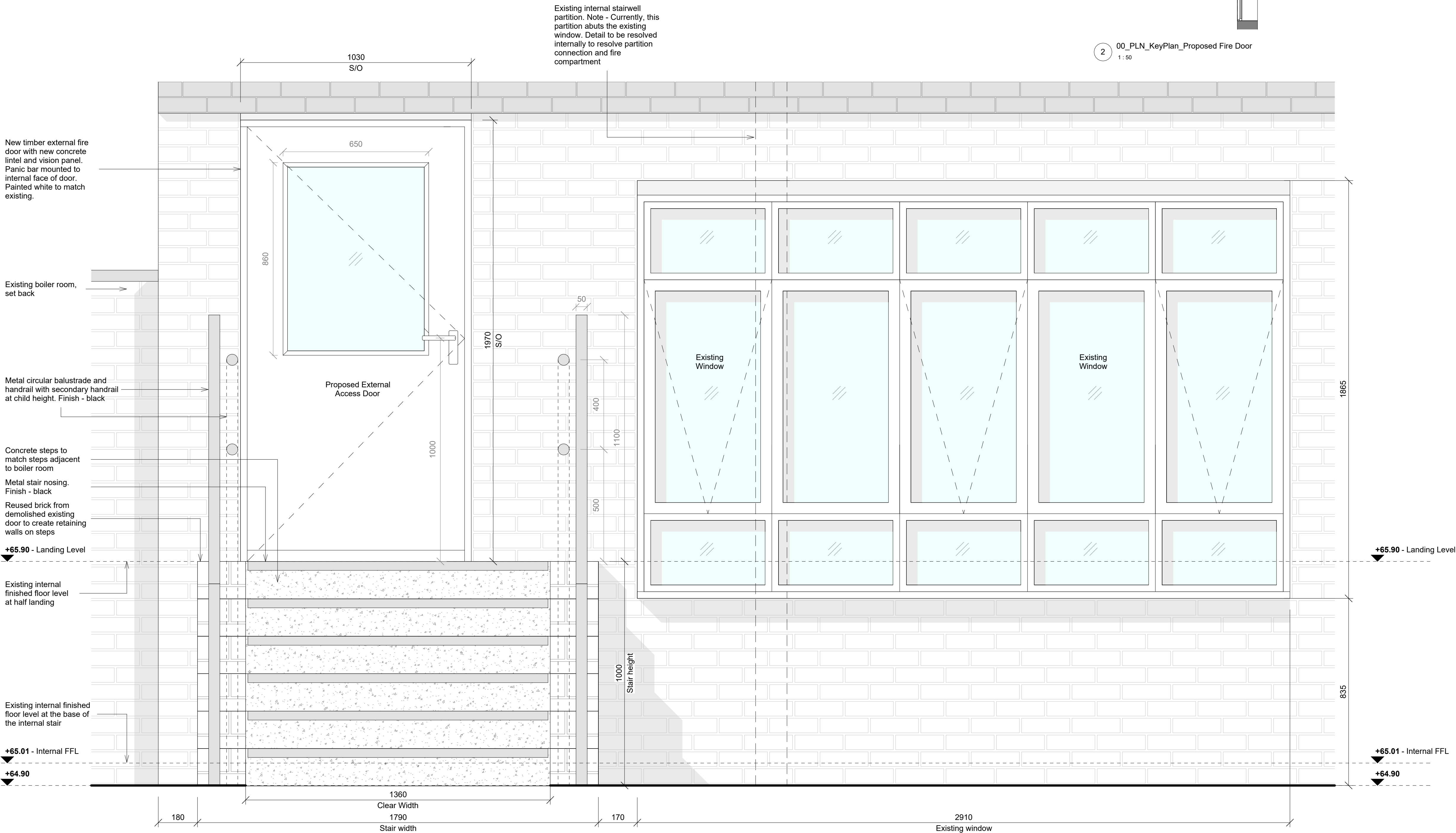
3 External Door - Proposed - Elevation A 1 : 10
