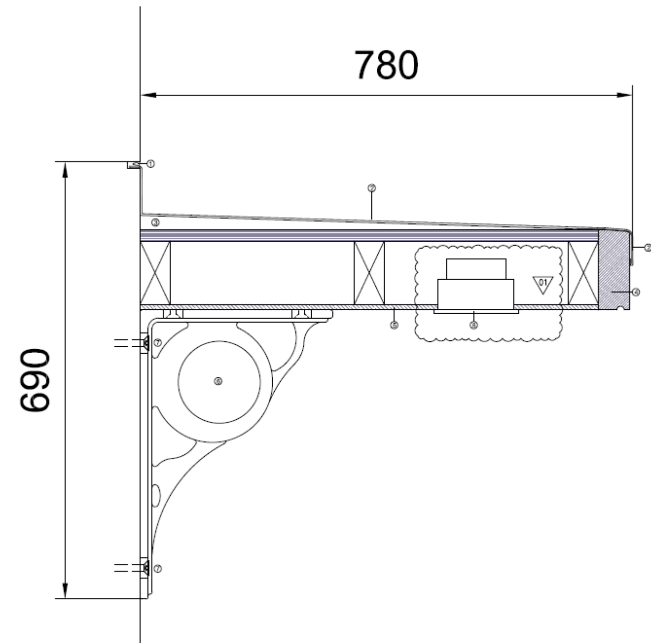
CANOPY SECTION A - A Scale 1:5
