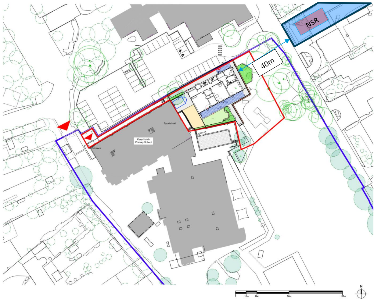
Figure 3-2: Proposed site plan with plant installation location and nearest NSR marked
