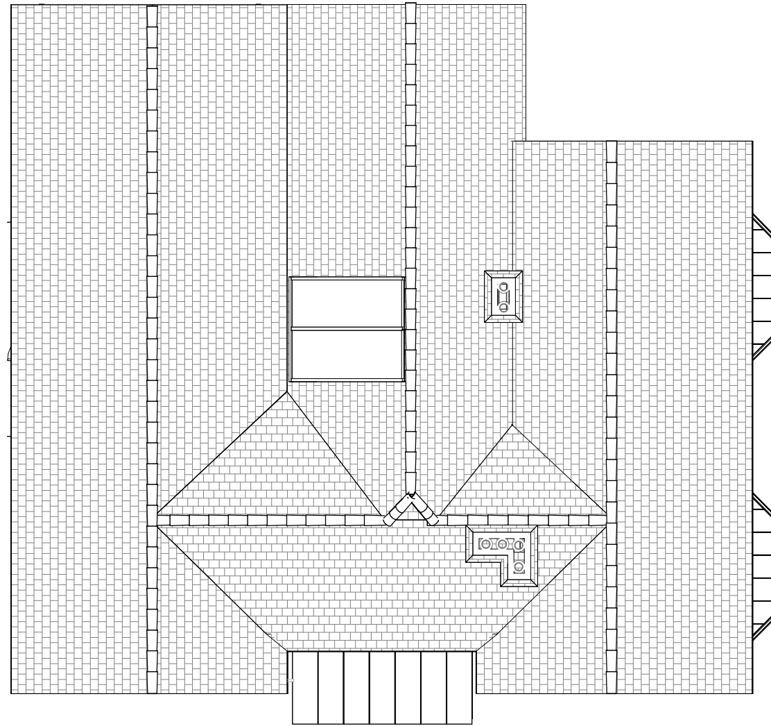
Roof Plan
