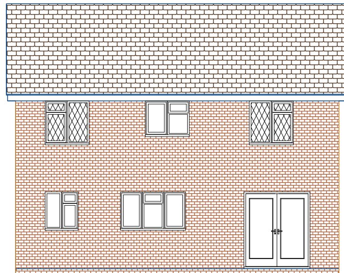
Proposed Rear Elevation (no change)
