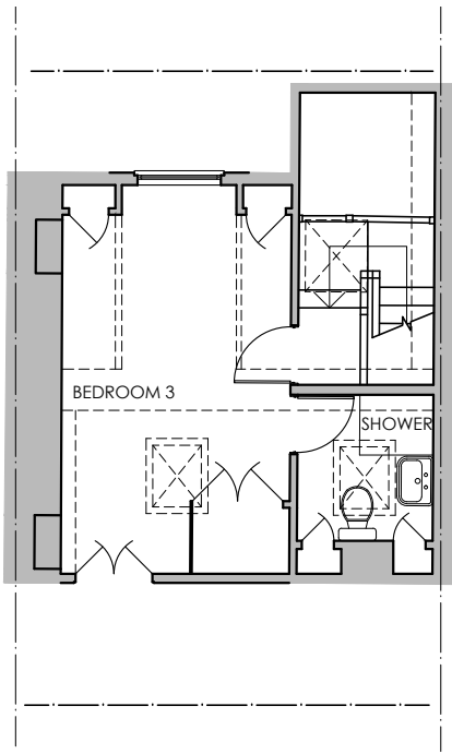
SECOND FLOOR PLAN 1:100
