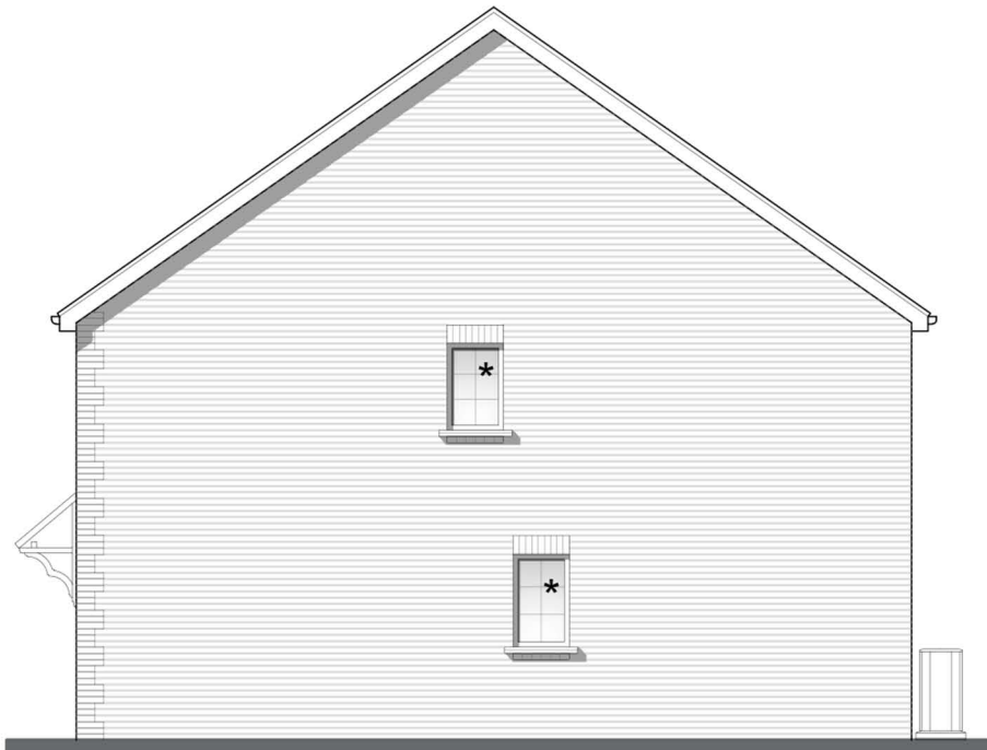
Elevation D
