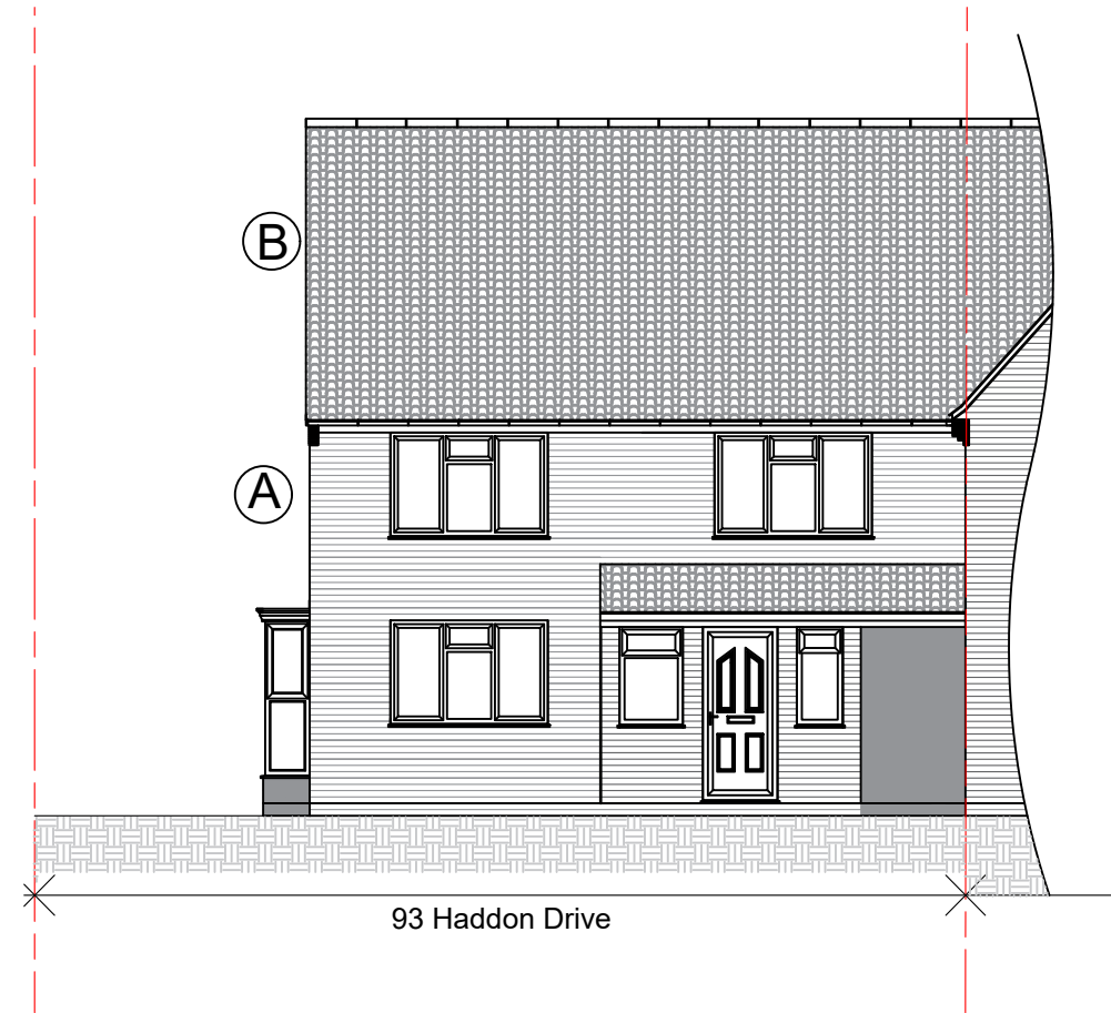
03 Existing Front Elevation HDAA3 SCALE: 1:100@A3
