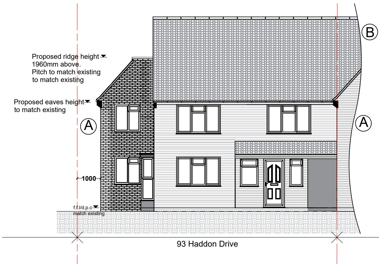
04 Proposed Front Elevation HDAA3 SCALE: 1:100@A3
