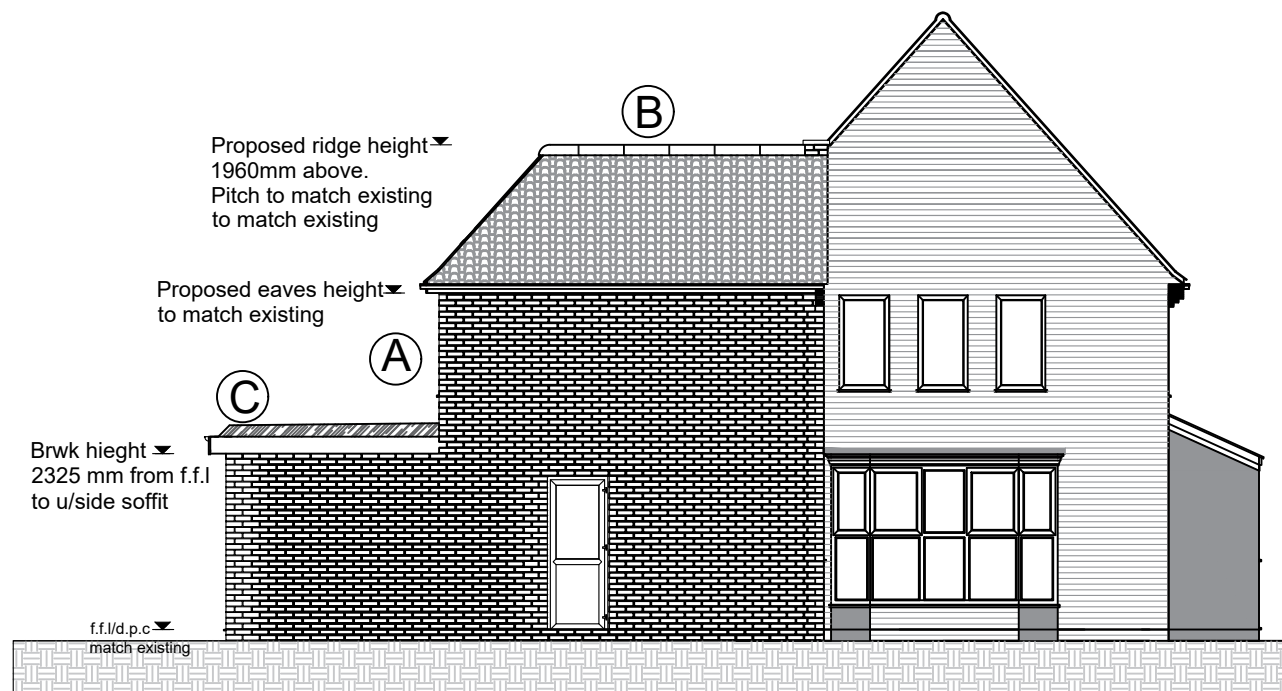
04 Proposed Front Elevation HDAA3 SCALE: 1:100@A3
