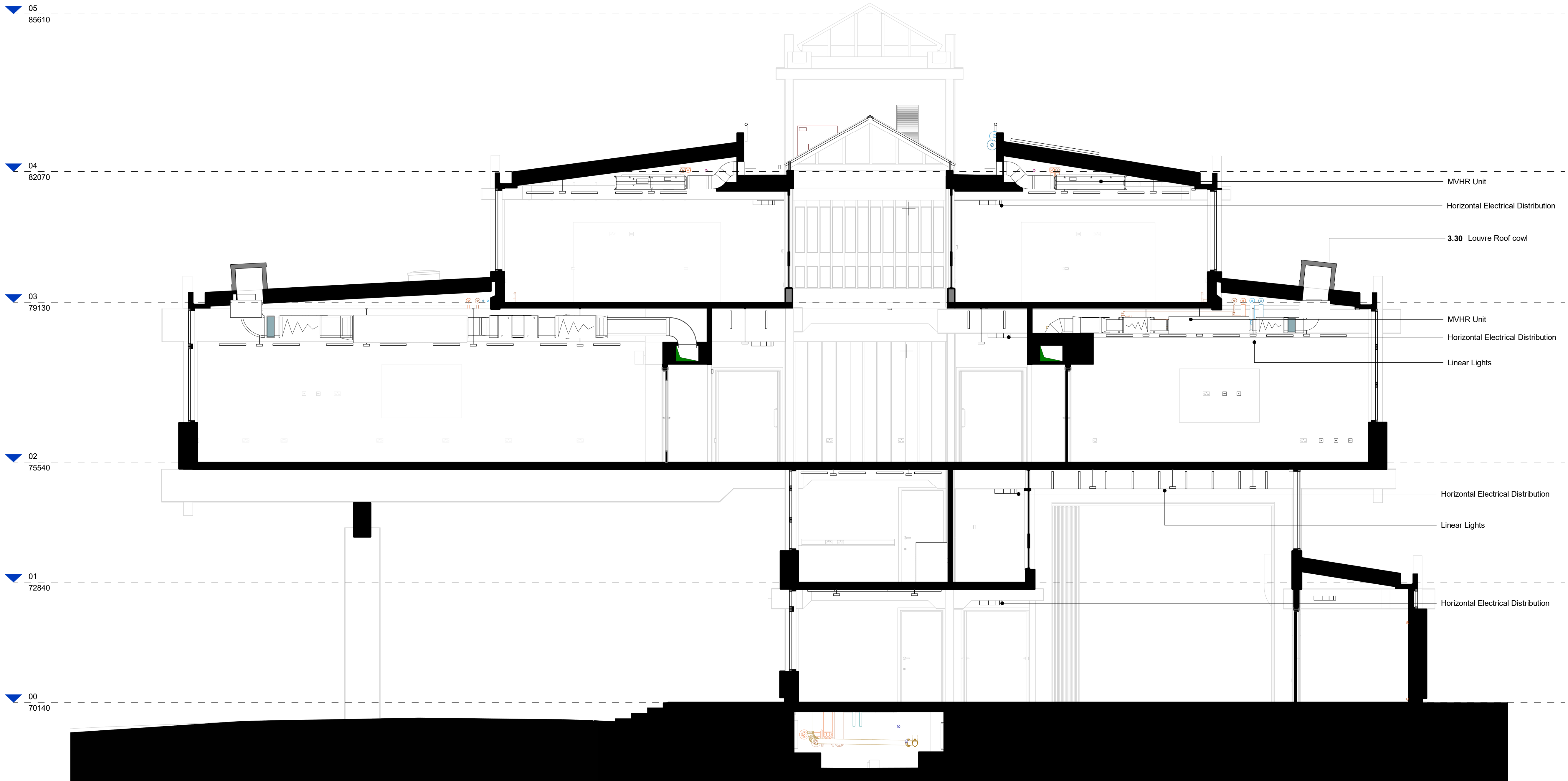
1 | 32300-Typical Section-Services Integration 1 : 50
