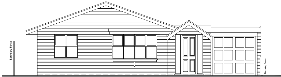
Front Elevation
