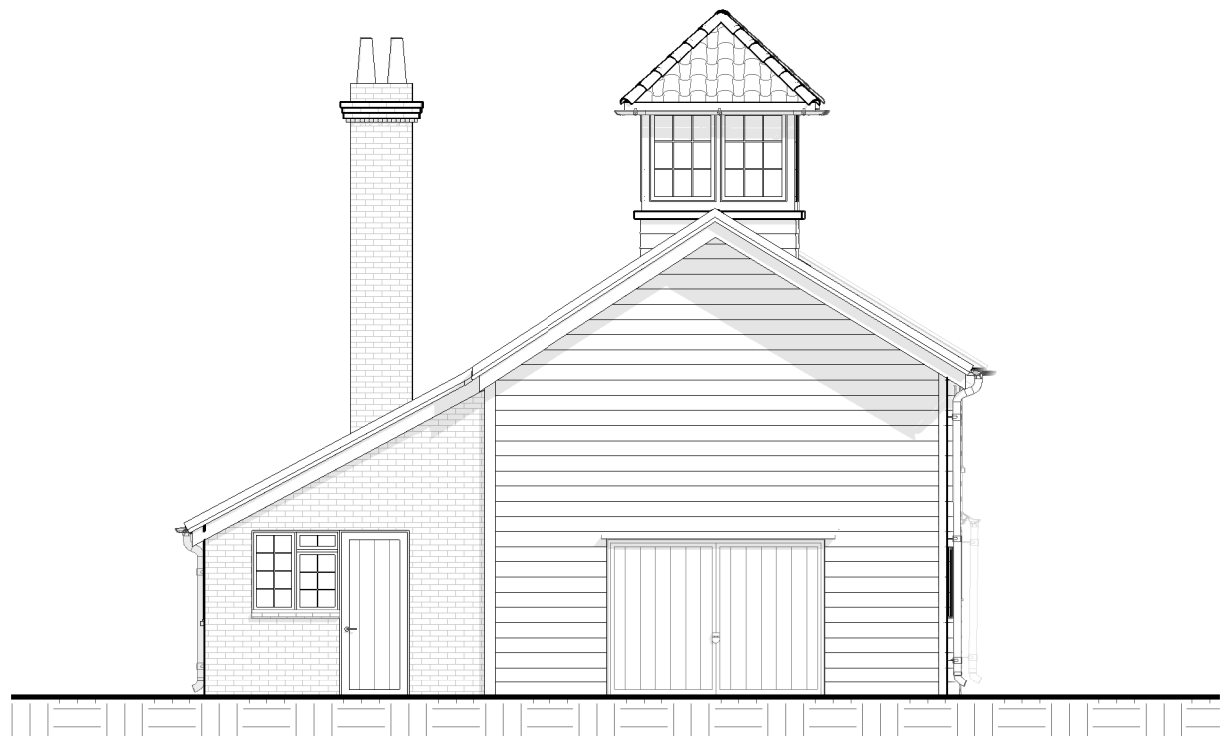
South-West Elevation
