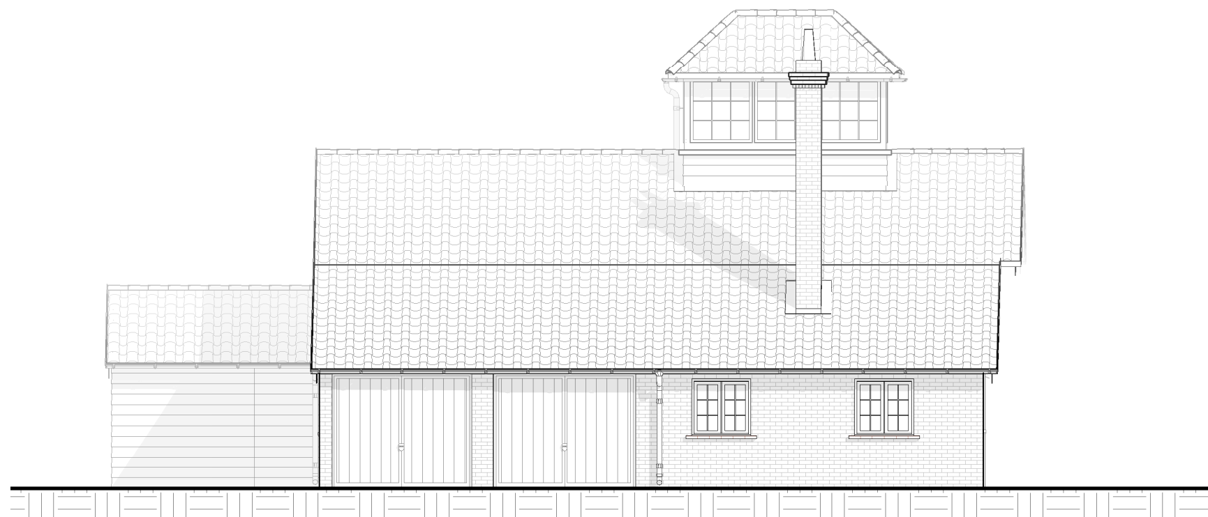
South-West Elevation
