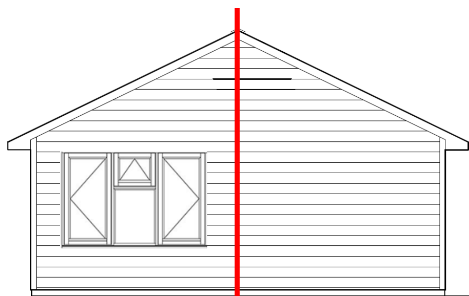
③ REAR ELEVATION
