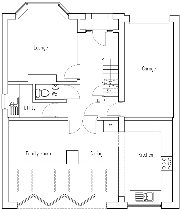
1:100 Existing Ground floor plan
