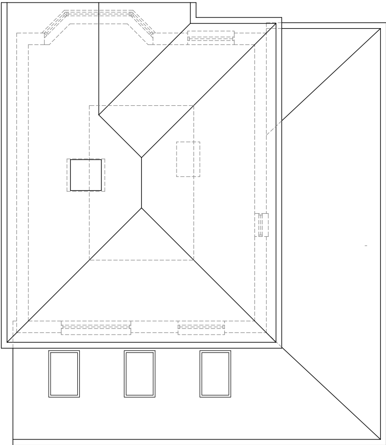
1:100 Existing Roof plan
