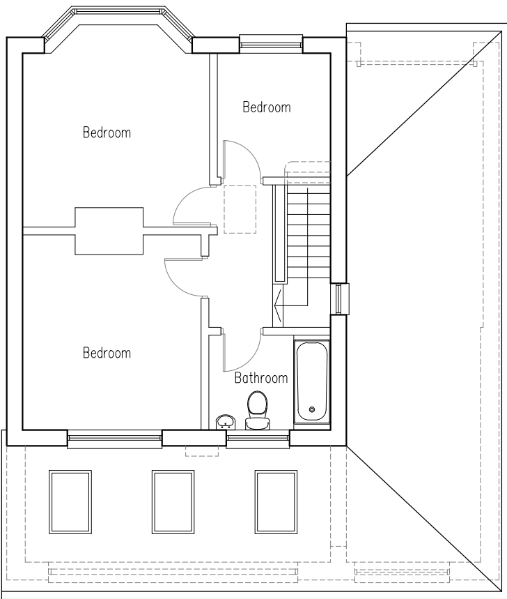
1:100 Existing First floor plan
