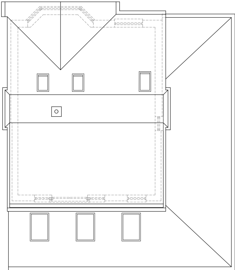
1:100 Proposed Roof plan
