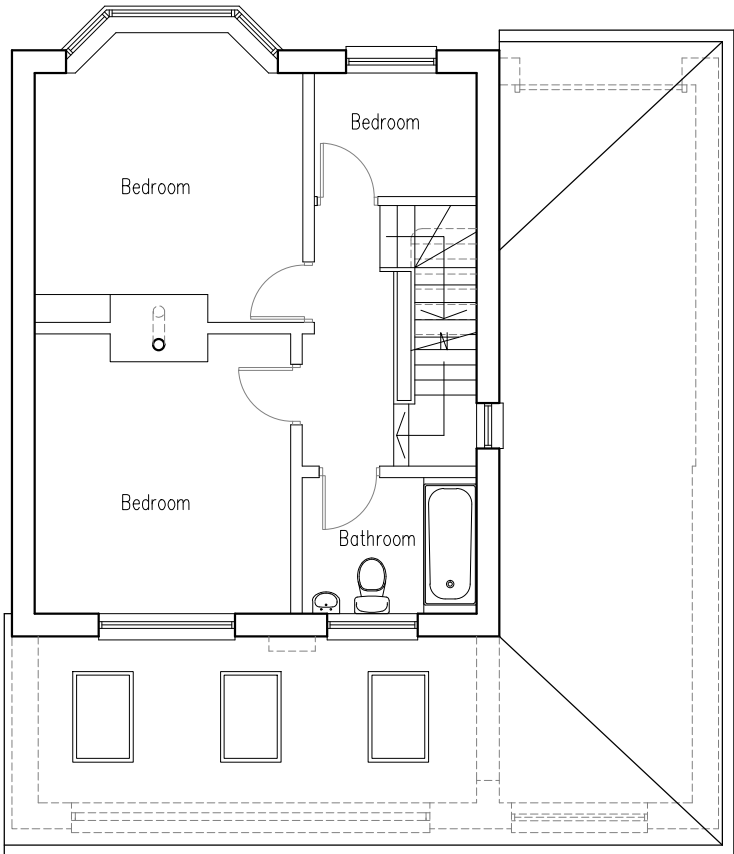
1:100 Proposed First floor plan
