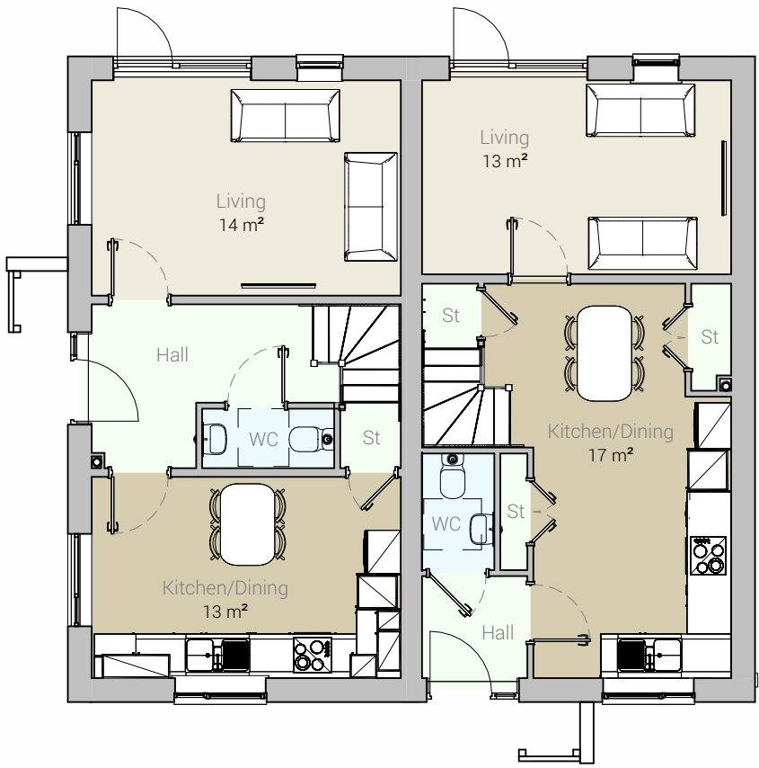
Ground Floor 1 : 100
