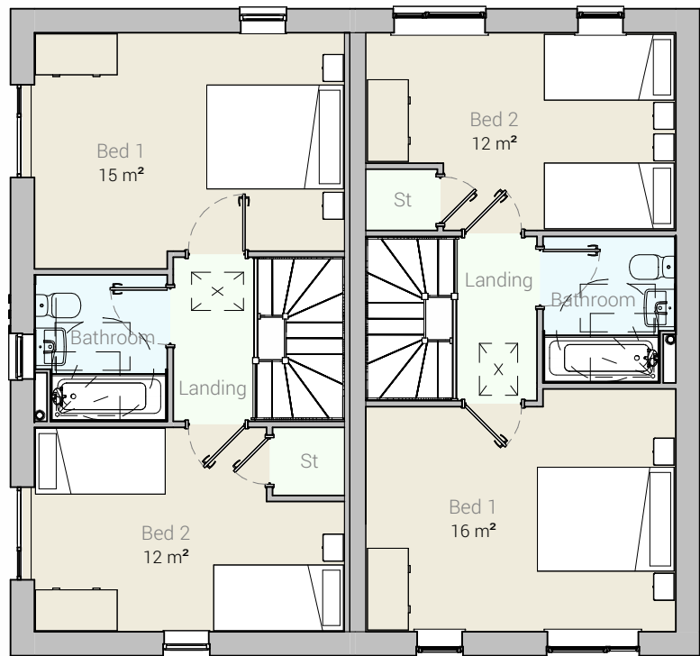
First Floor 1 : 100
