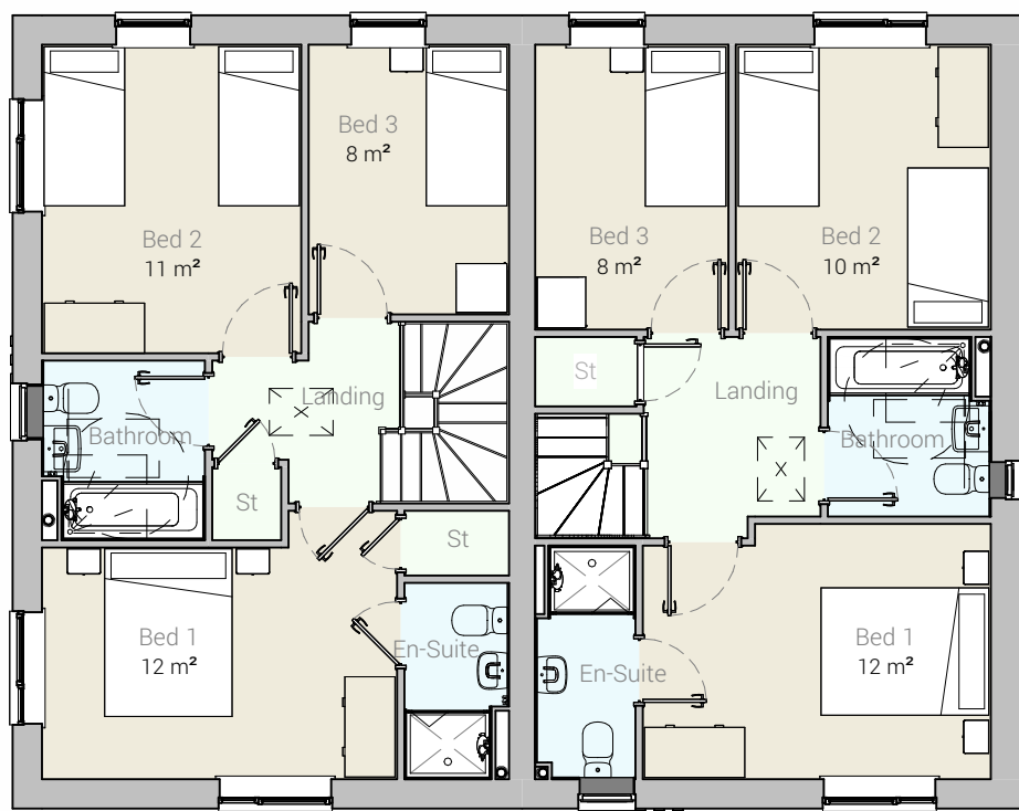
First Floor 1 : 100
