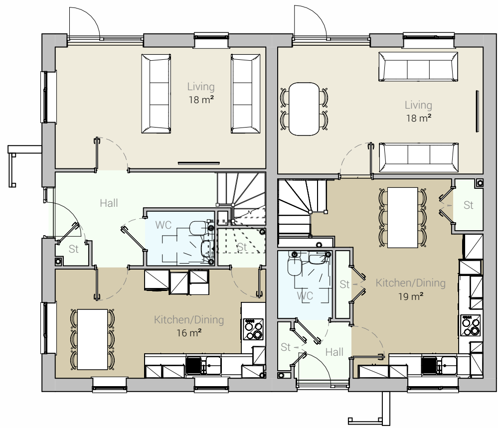
Ground Floor 1 : 100
