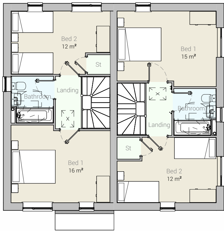
First Floor 1 : 100
