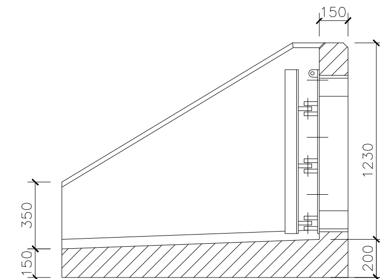
ALTHON (SFA 10C) HEADWALL (INLET) DETAIL (SCALE 1:20)
