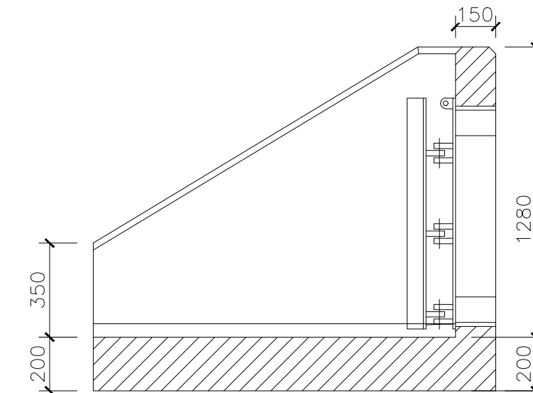
ALTHON (SFA 11C) HEADWALL (OUTLET) DETAIL (SCALE 1:20)
