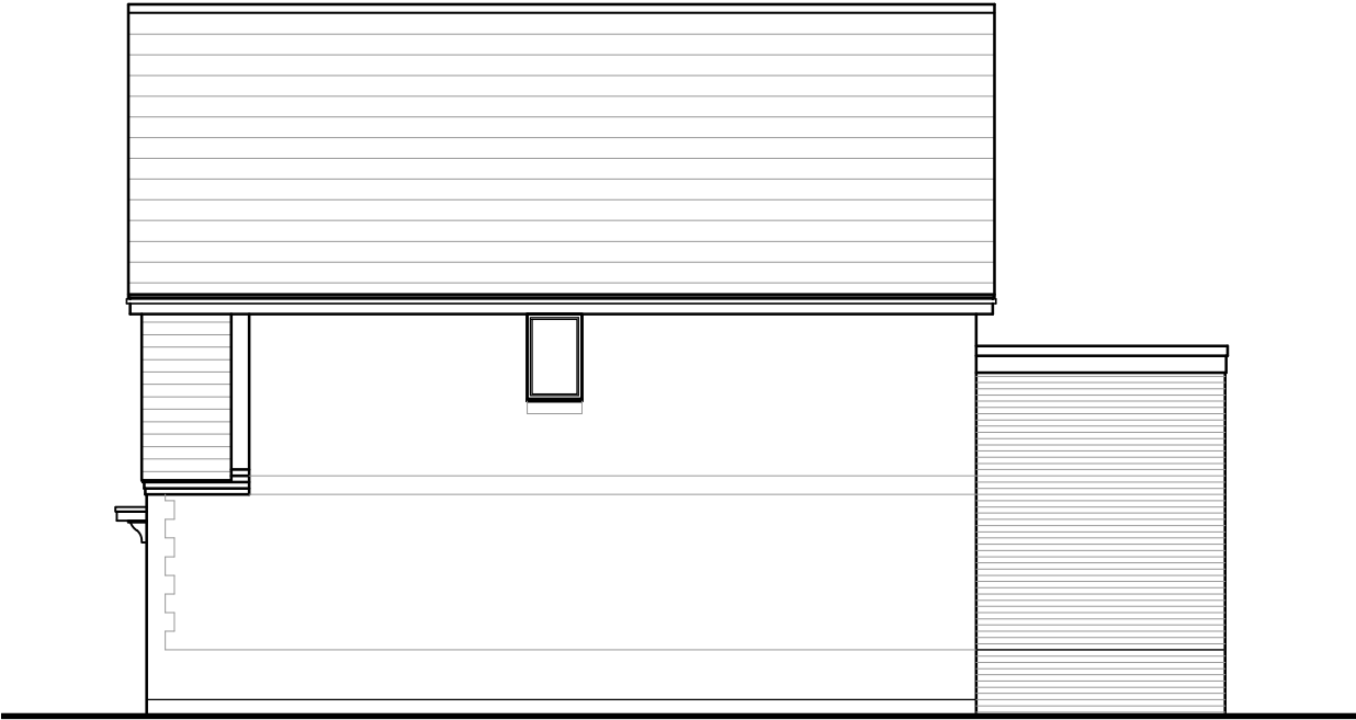
EAST ELEVATION
