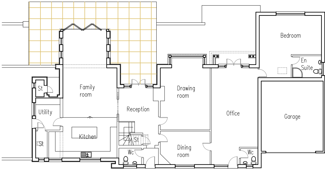
1:200 Proposed Ground floor plan
