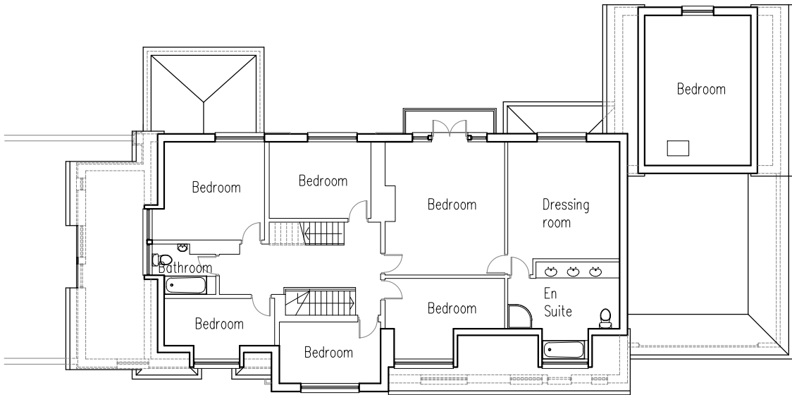
1:200 Proposed First floor plan
