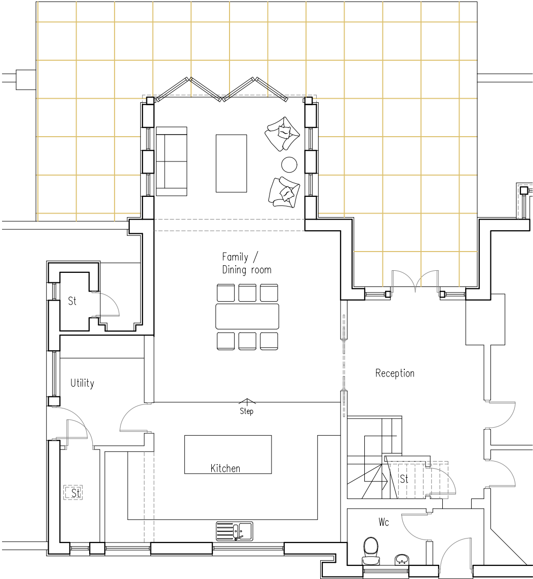
1:100 Proposed Part Ground floor plan
