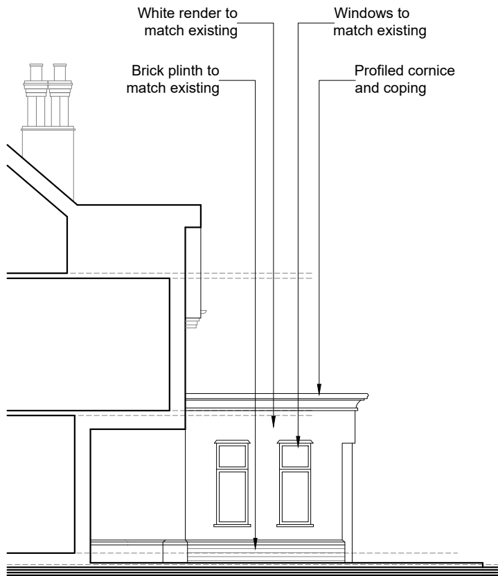
1:100 Proposed Part Rh side Elevation / Section
