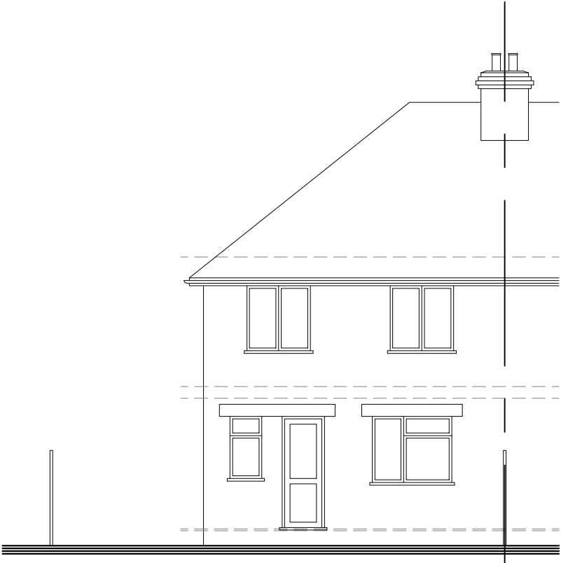
1:100 Existing Rear Elevation
