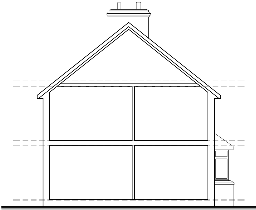
1:100 Existing Lh side Elevation / Section
